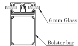
Roof Bar & Sheet Section
