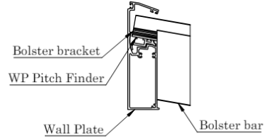
Wall Plate & Roof Bar Section
