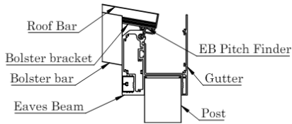
Eaves Beam Roof Bar & Post Section
