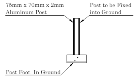
Base & Post Connection Information
